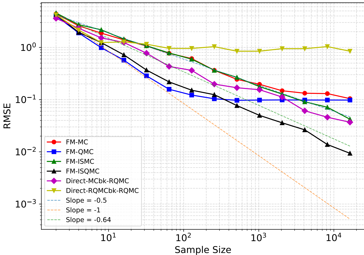
30D GMM, Second moment: 4 FM + 2 direct baselines
