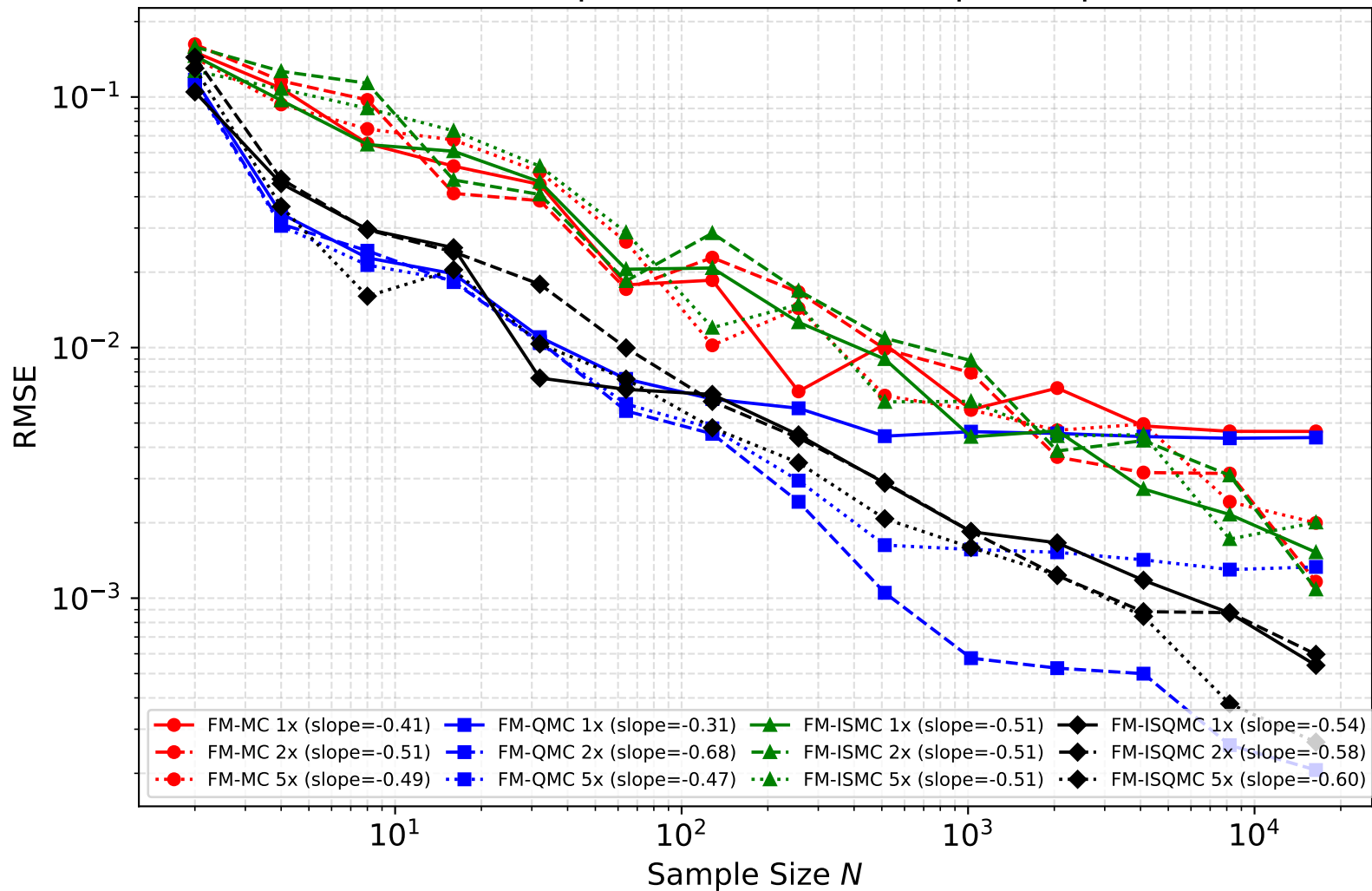
30D GMM, Complex f: 1x / 2x / 5x ckpt comparison
