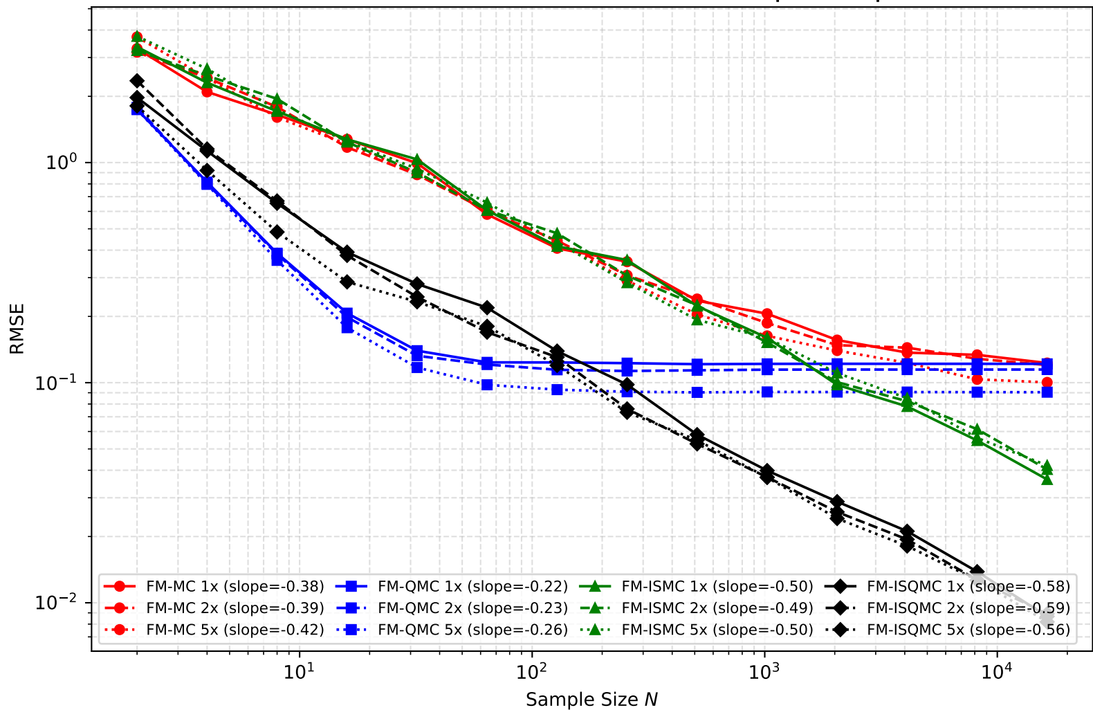
30D GMM, First moment: 1x / 2x / 5x ckpt comparison
