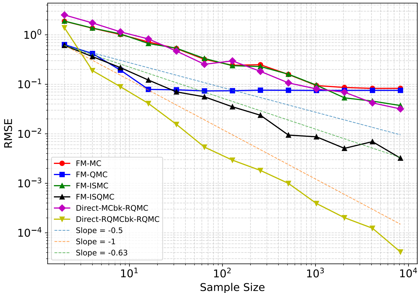
2D GMM, First moment: 4 FM + 2 direct baselines
