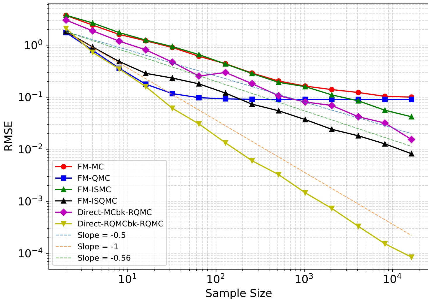
30D GMM, First moment: 4 FM + 2 direct baselines
