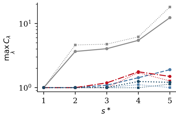
(b) the cut ratio (dotted: (4p \text{Gap})^{-1} )
