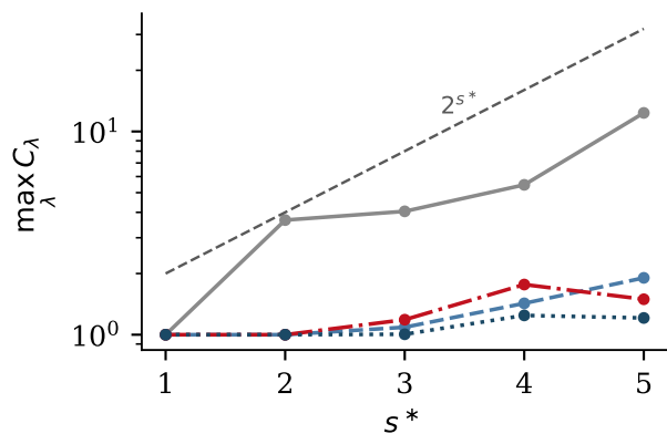
(d) the cut ratio does not grow with s^*
