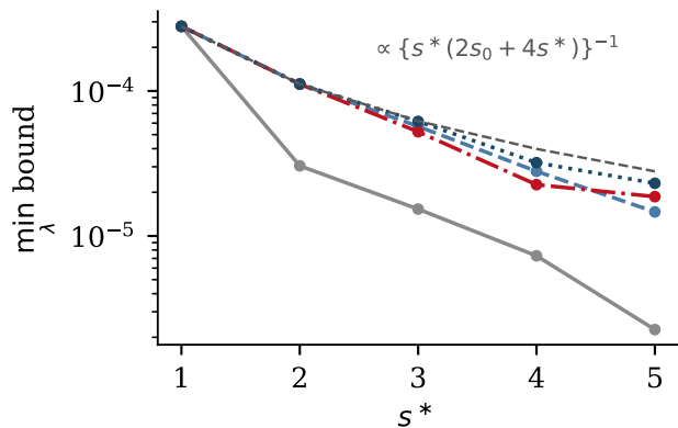
(c) the certificate decays polynomially
