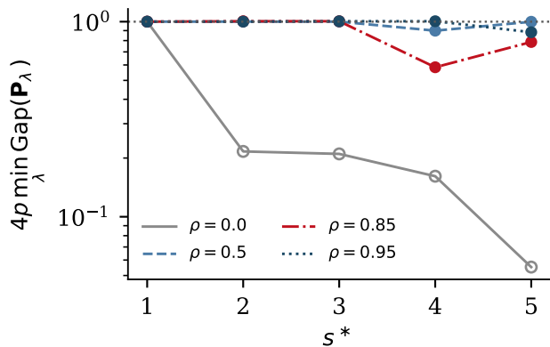
(a) the exact gap; open marker: (B2) fails
