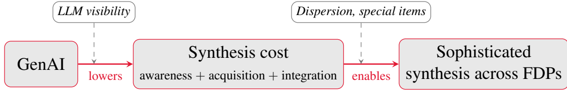
FIGURE 1. Theoretical Framework
