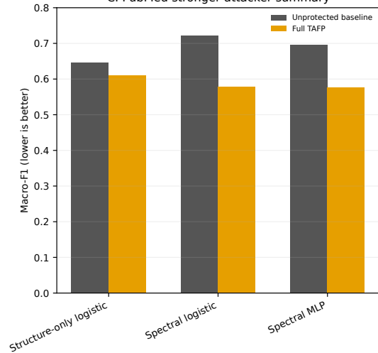
C. PubMed stronger attacker summary
