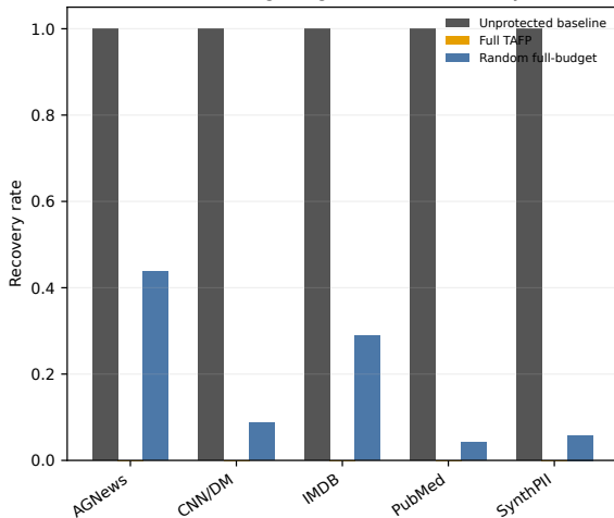
B. Fixed-edge original relation recovery
