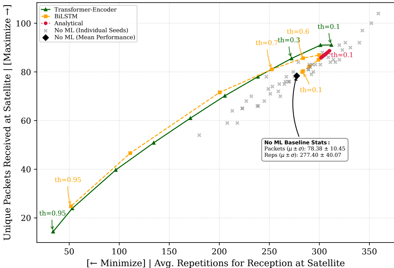
Pareto Frontier of Packets and Repetitions across Decision Thresholds
