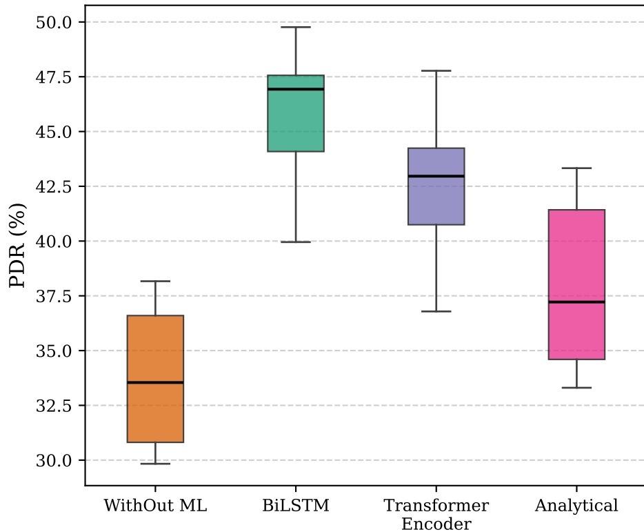
(a) Packet Delivery Ratio (PDR)
