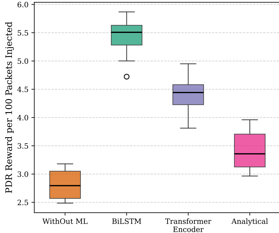
(b) PDR Efficiency
