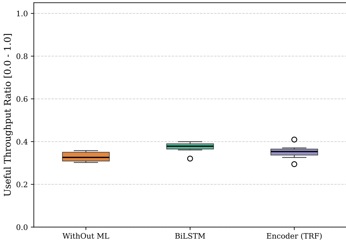
Link Transmission Efficiency ( \eta )
