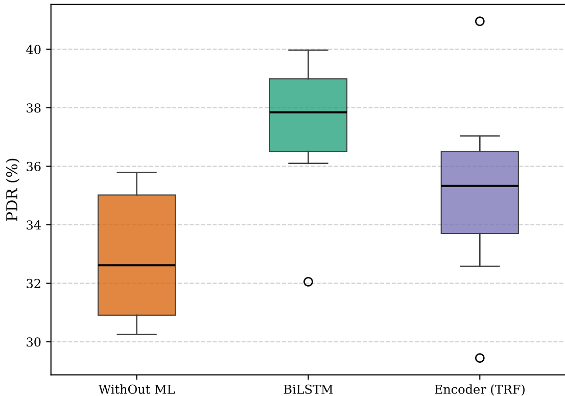
Packet Delivery Ratio (PDR) Robustness Analysis
