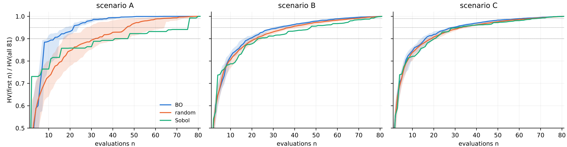
M = 4 hypervolume recovery: median and 20-80 % band (dotted: 90/95/99 %)
