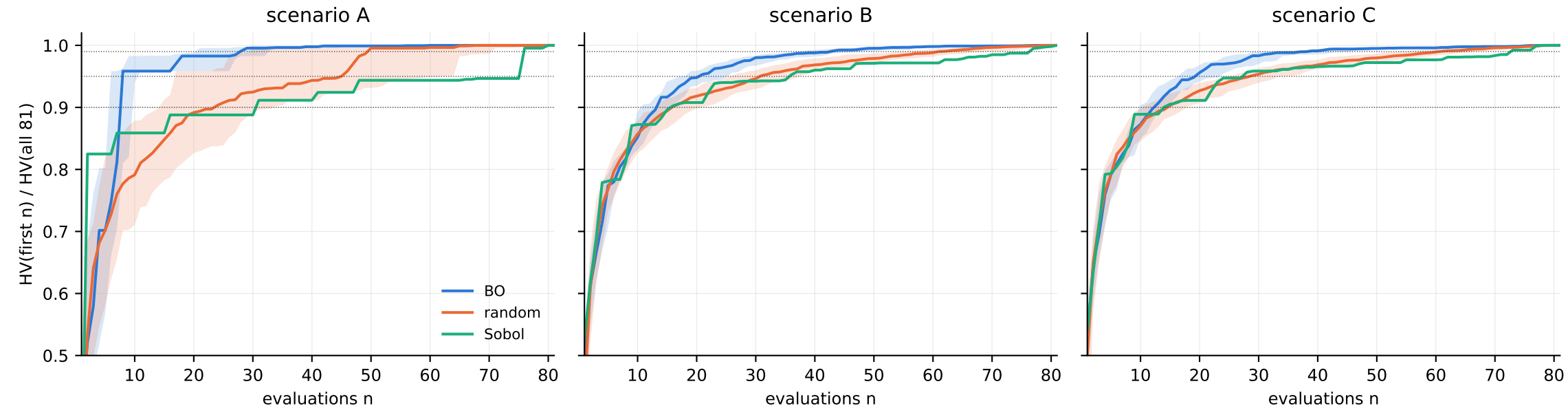
Cost-shed ( M = 2 ) hypervolume recovery: median and 20-80 % band
