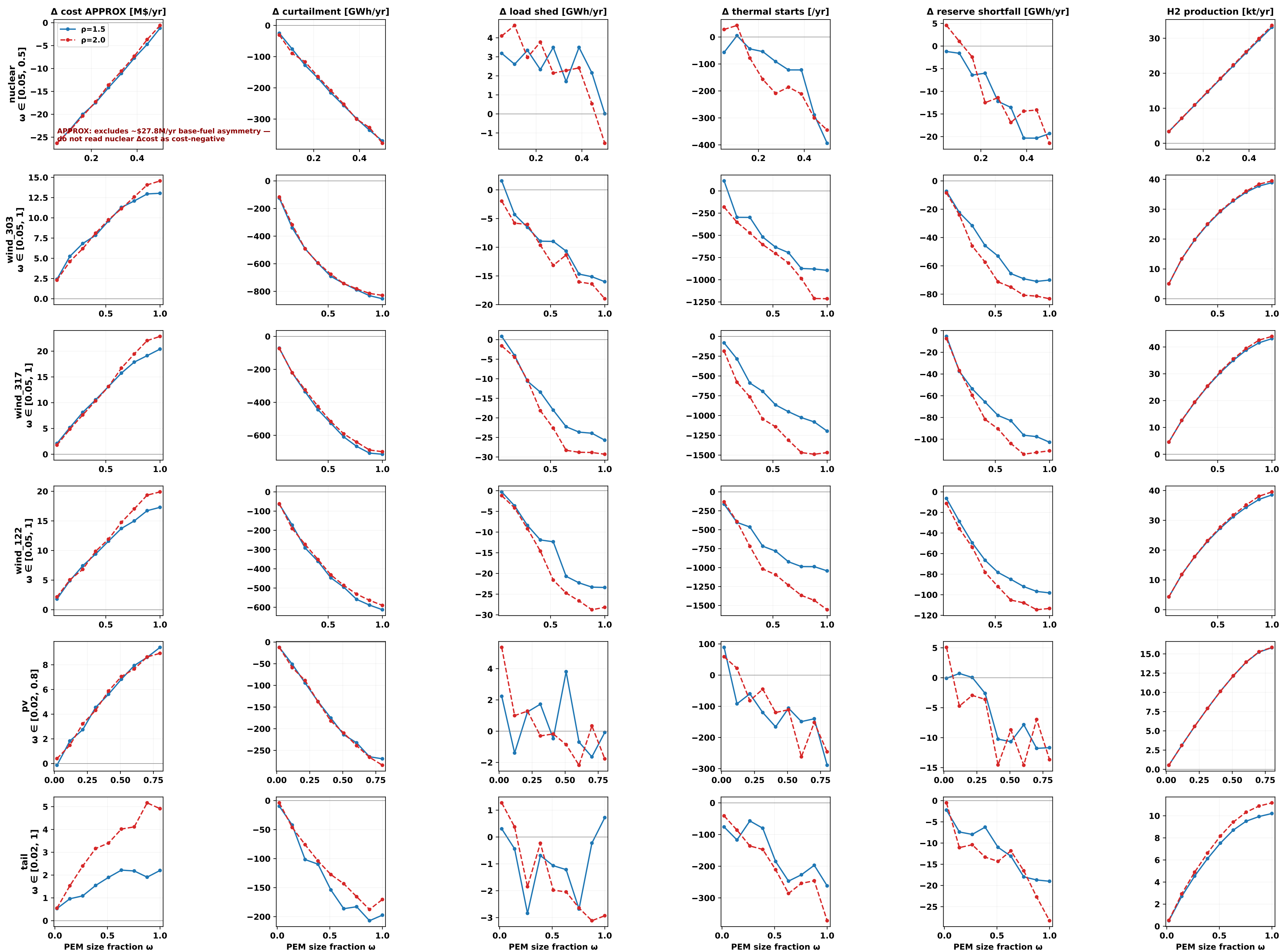
Per-tier OAT \omega sweeps: g(\omega) by tier \times metric ( \Delta vs base; negative = improvement)
