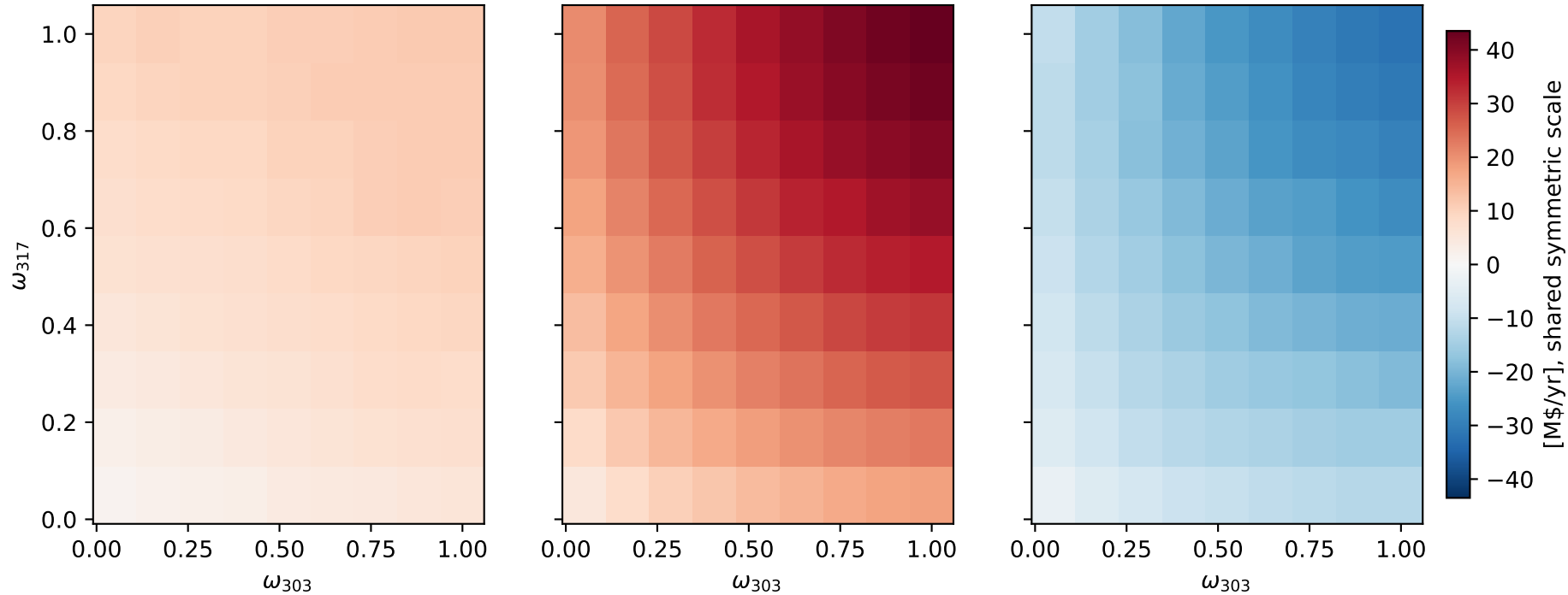
Cost decomposition, scenario A ( \rho_{H2} = 1.0 $/kg): the APPROX-column sign structure is raw minus synthetic bid cost raw \Delta cost = total - base K_{syn} (synthetic bid cost) APPROX = raw - K_{syn}
