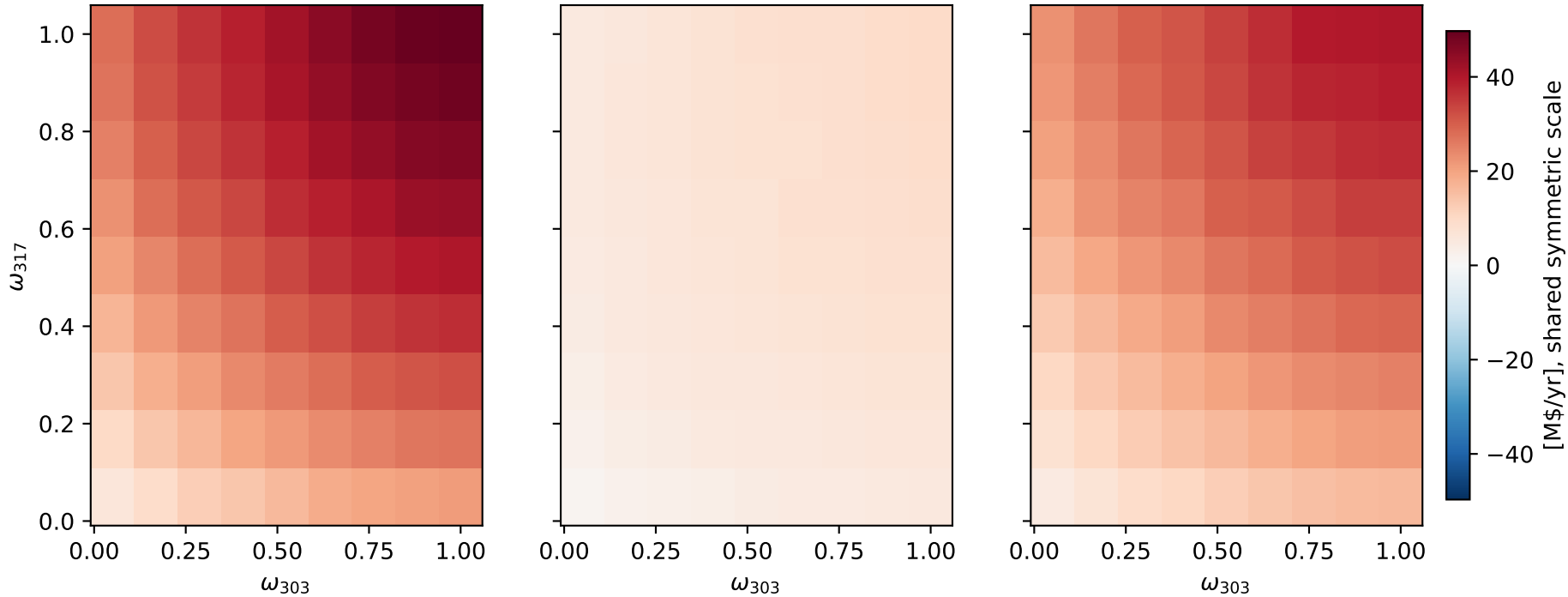
Cost decomposition, scenario B ( \rho_{H2} = 1.5 $/kg): the APPROX-column sign structure is raw minus synthetic bid cost raw \Delta\text{cost} = \text{total} - \text{base} K_{syn} (synthetic bid cost) APPROX = raw - K_{syn}
