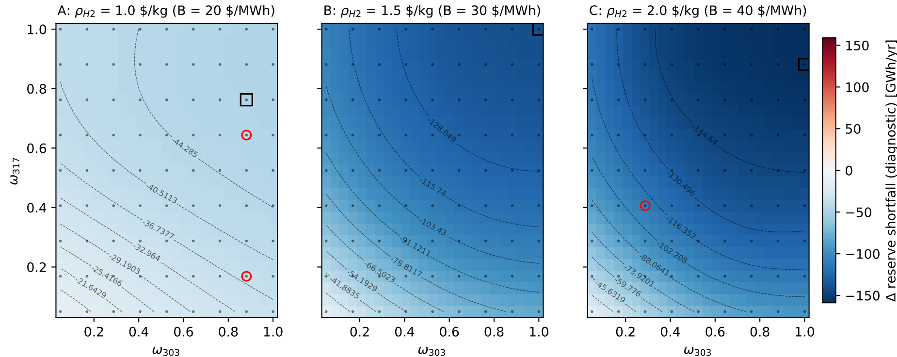
\Delta reserve shortfall (diagnostic) [GWh/yr] on the 303x317 pair grid (blue = improvement vs base)
