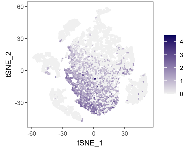
KCNE2 in the tumor-only t-SNE
