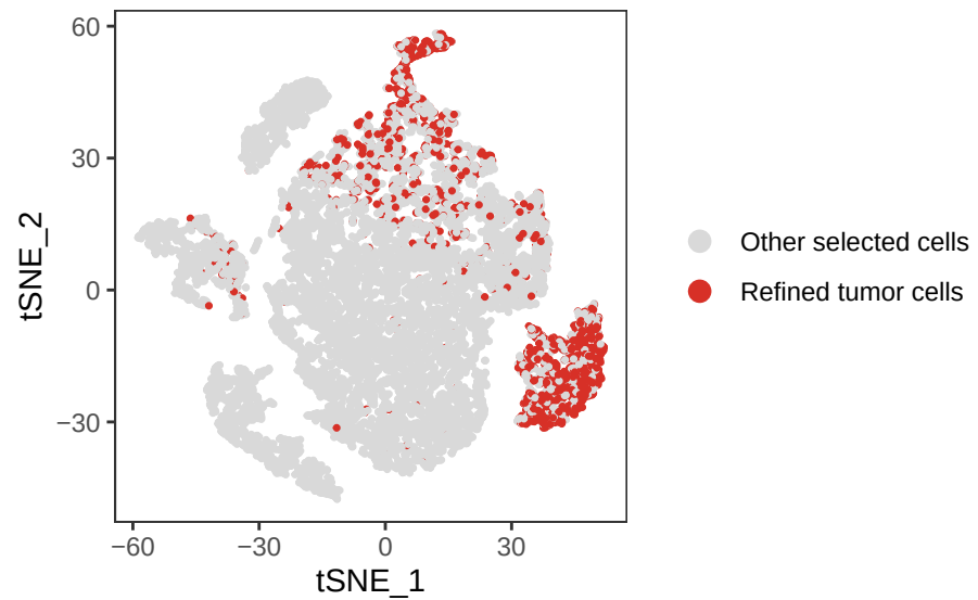
Global gastric t-SNE Refined markers + CNV tumor compartment
