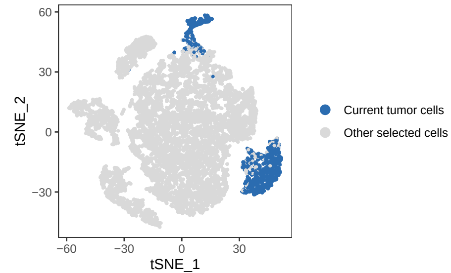
Global gastric t-SNE Current tumor compartment
