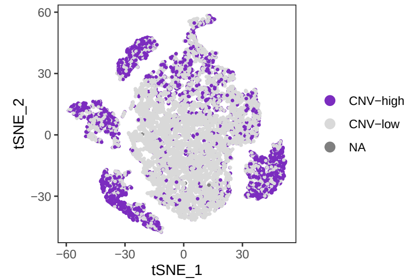
Global gastric t-SNE CNV-high cells
