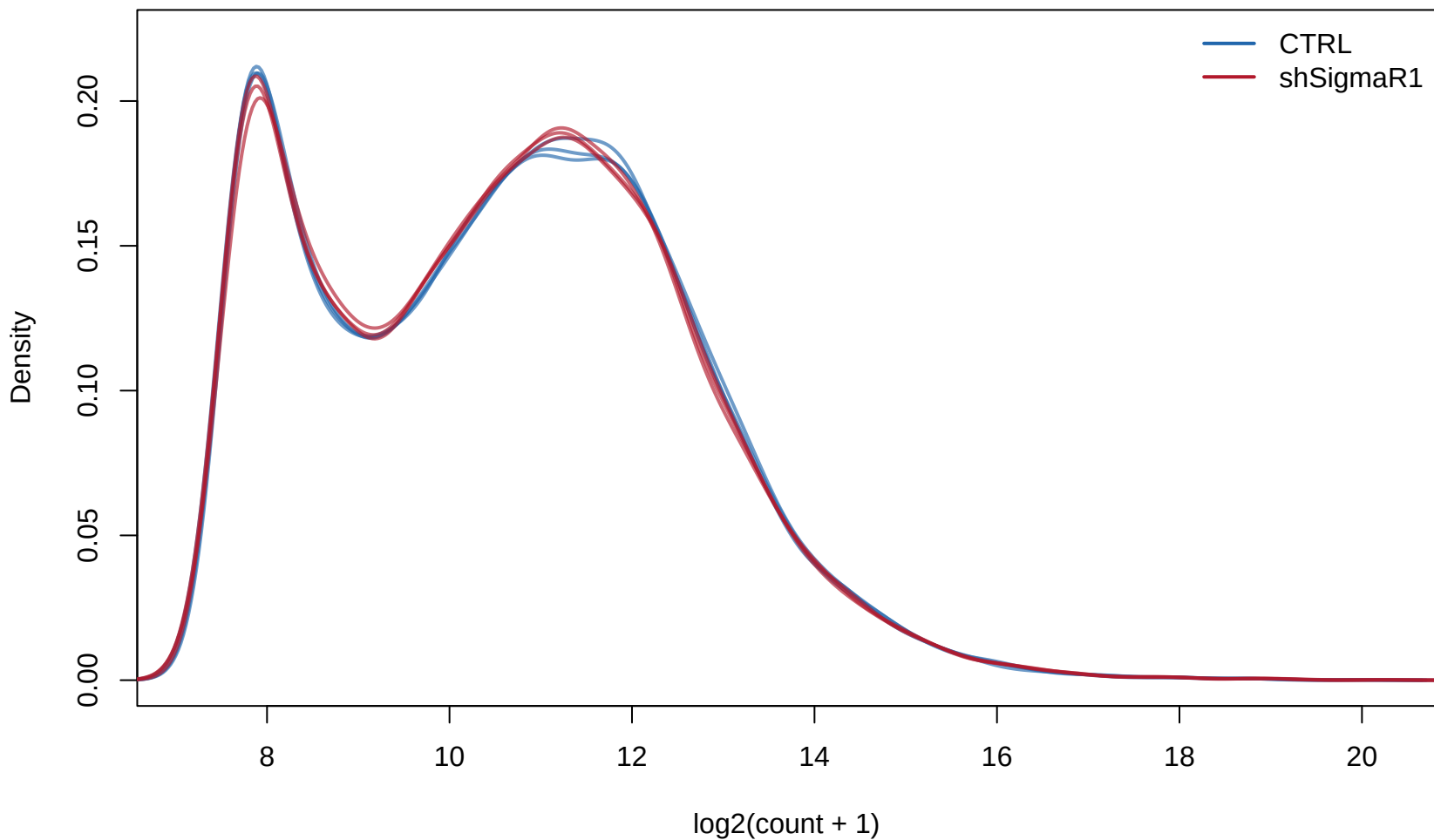
Per-sample density curves
