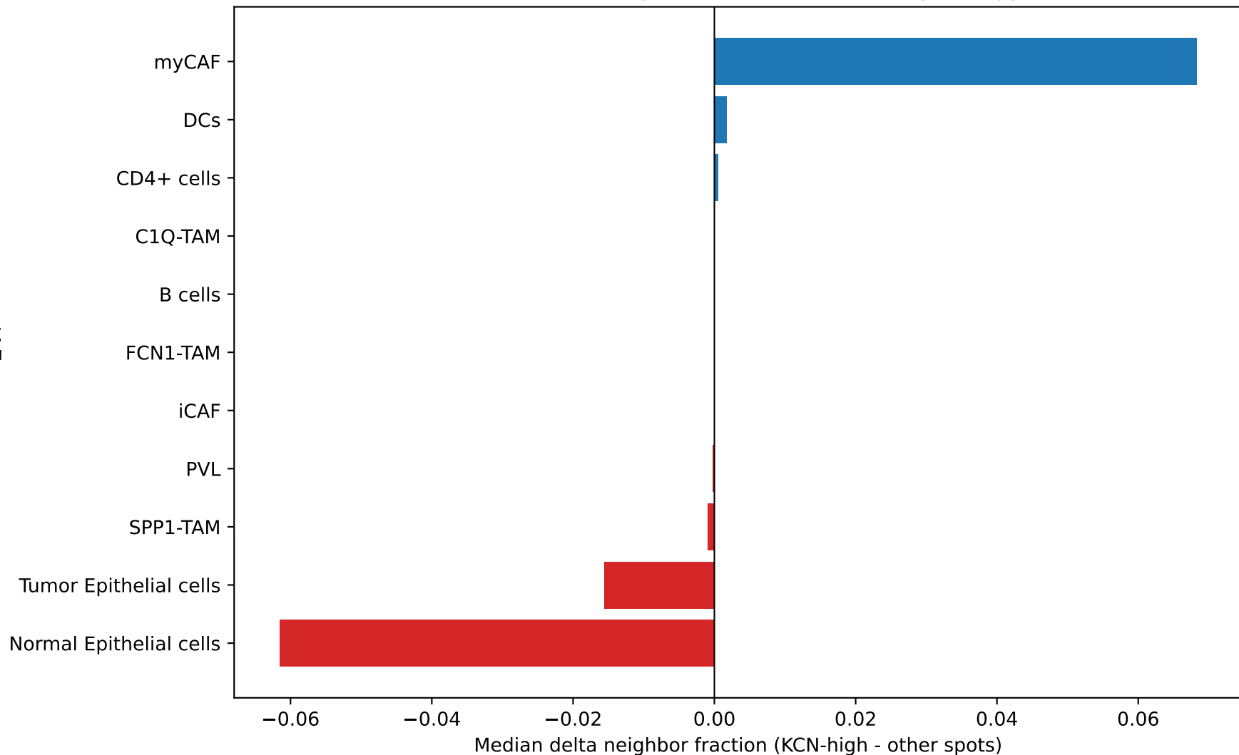
KCNAB2: KNN neighborhood enrichment by cell type
