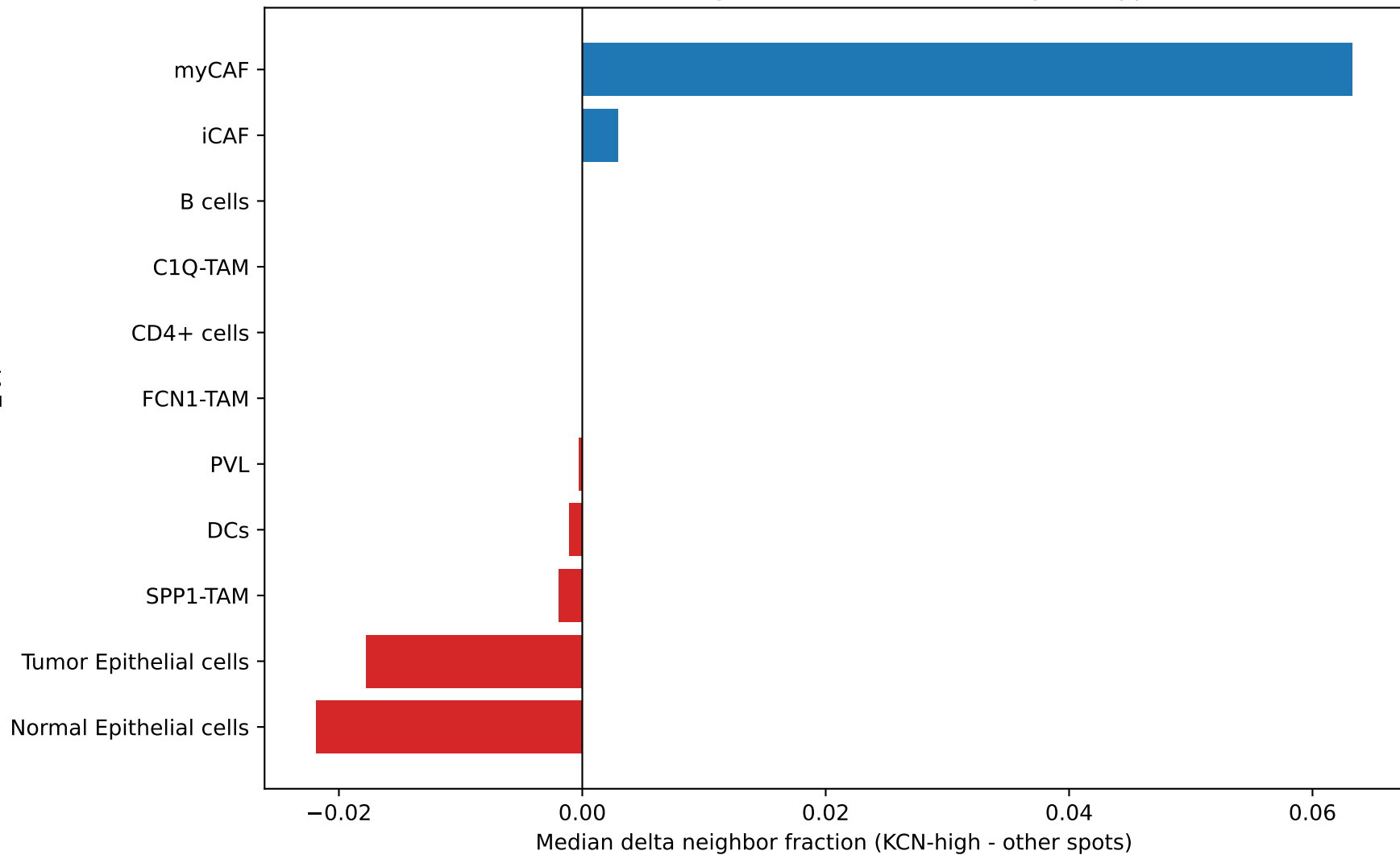
KCND2: KNN neighborhood enrichment by cell type
