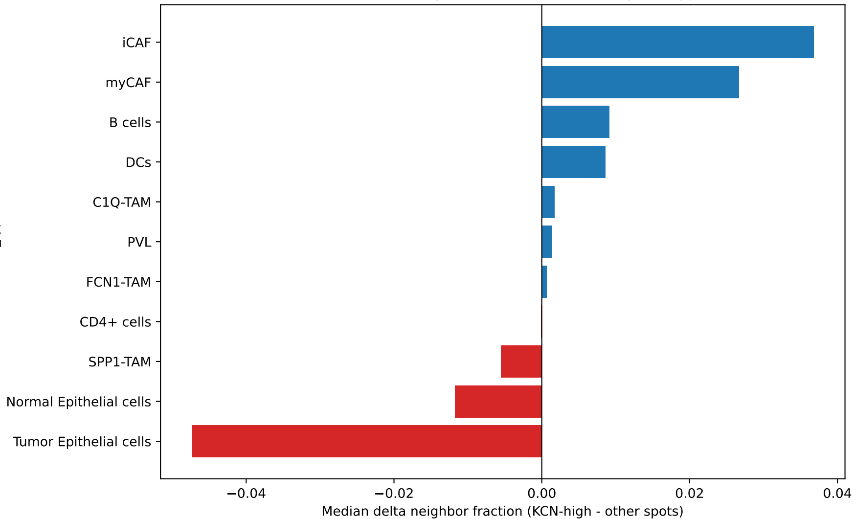
KCNK17: KNN neighborhood enrichment by cell type
