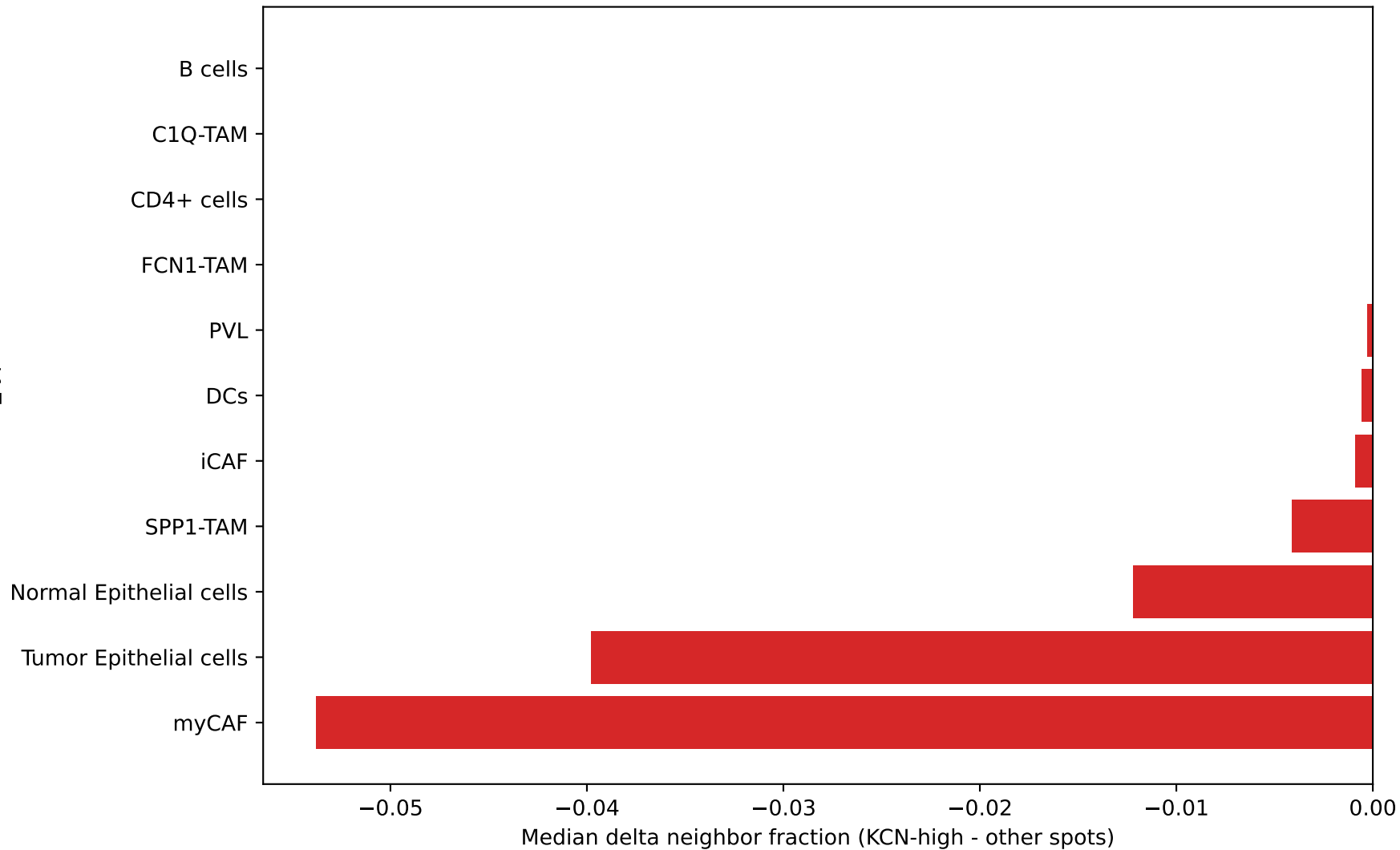
KCNK3: KNN neighborhood enrichment by cell type
