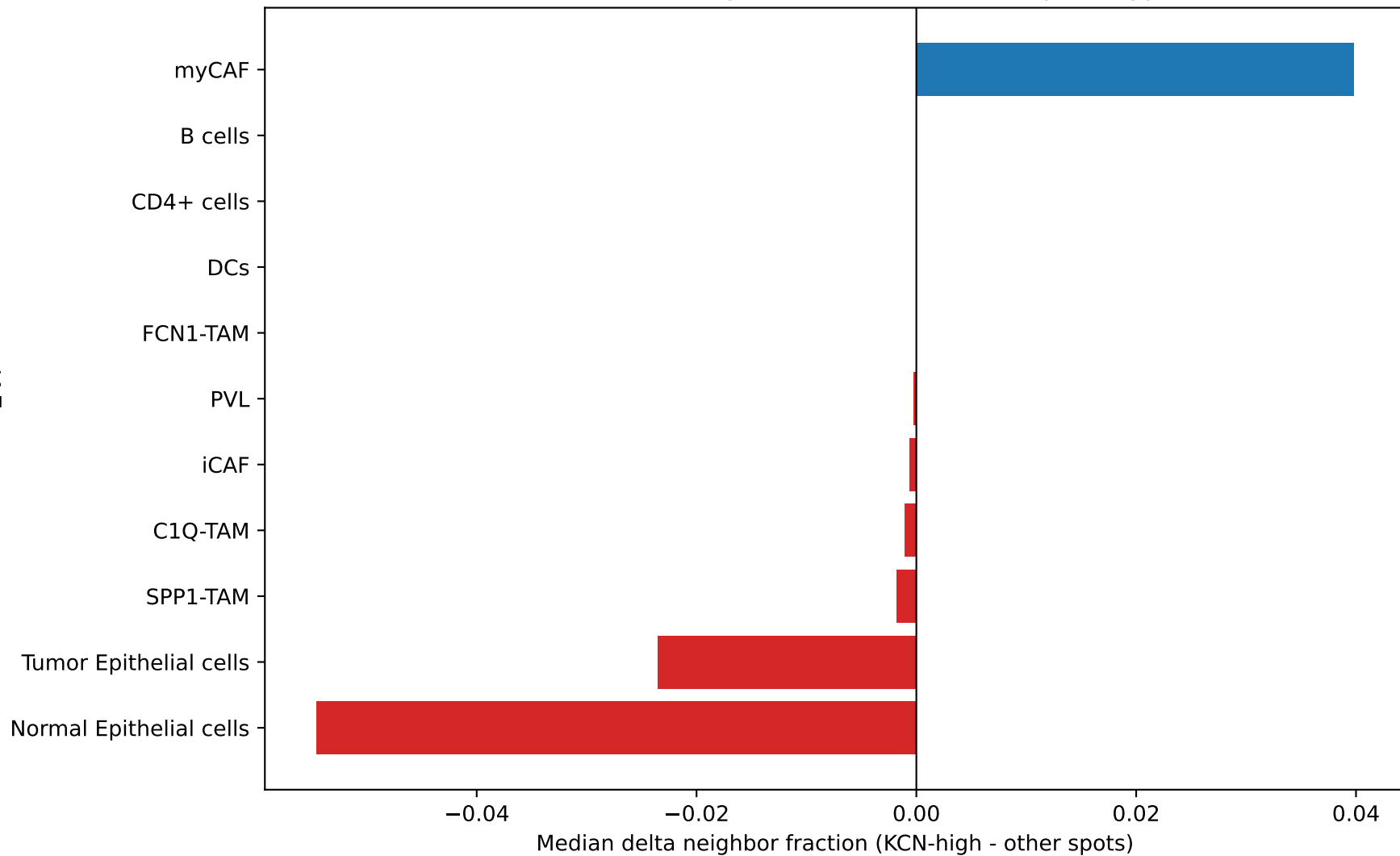
KCNMB4: KNN neighborhood enrichment by cell type
