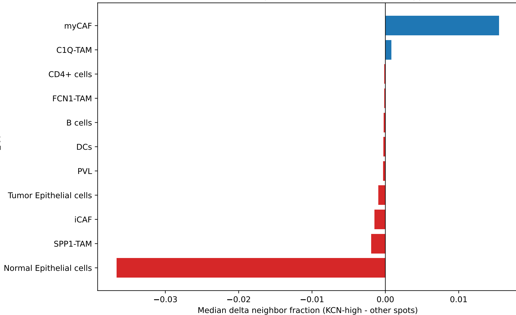
KCNQ4: KNN neighborhood enrichment by cell type
