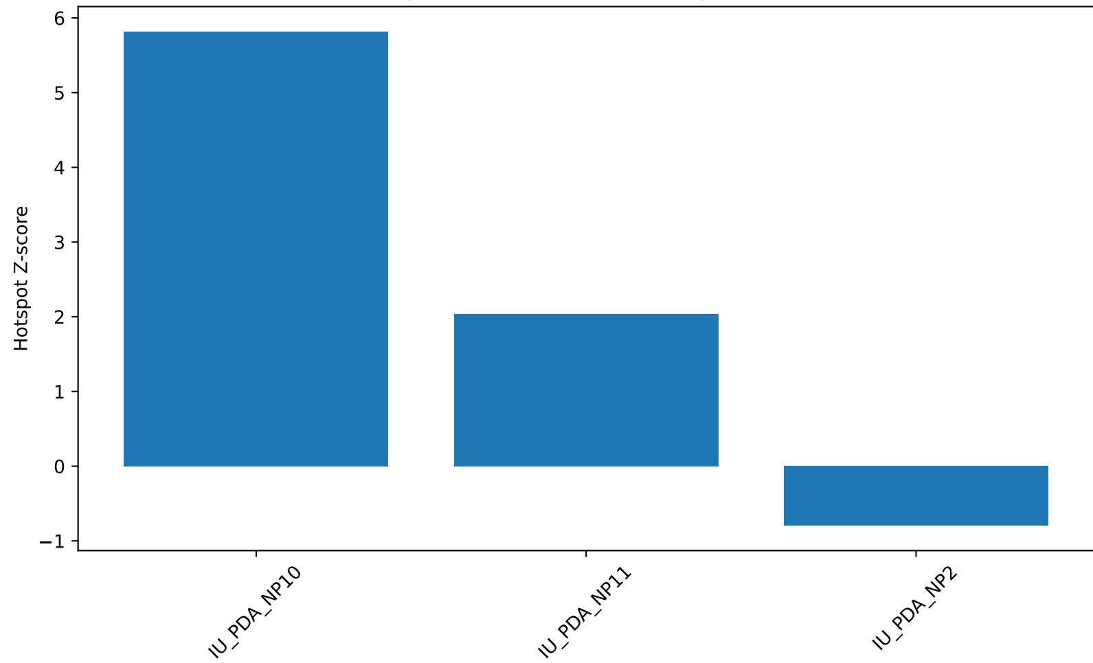
KCNC4 Hotspot Z-score across normal pancreas sections
