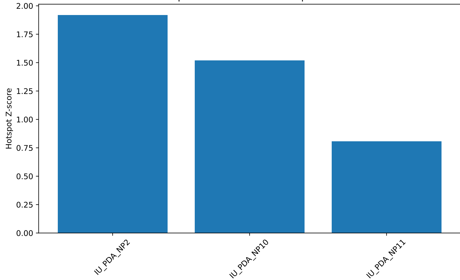
KCNMB4 Hotspot Z-score across normal pancreas sections
