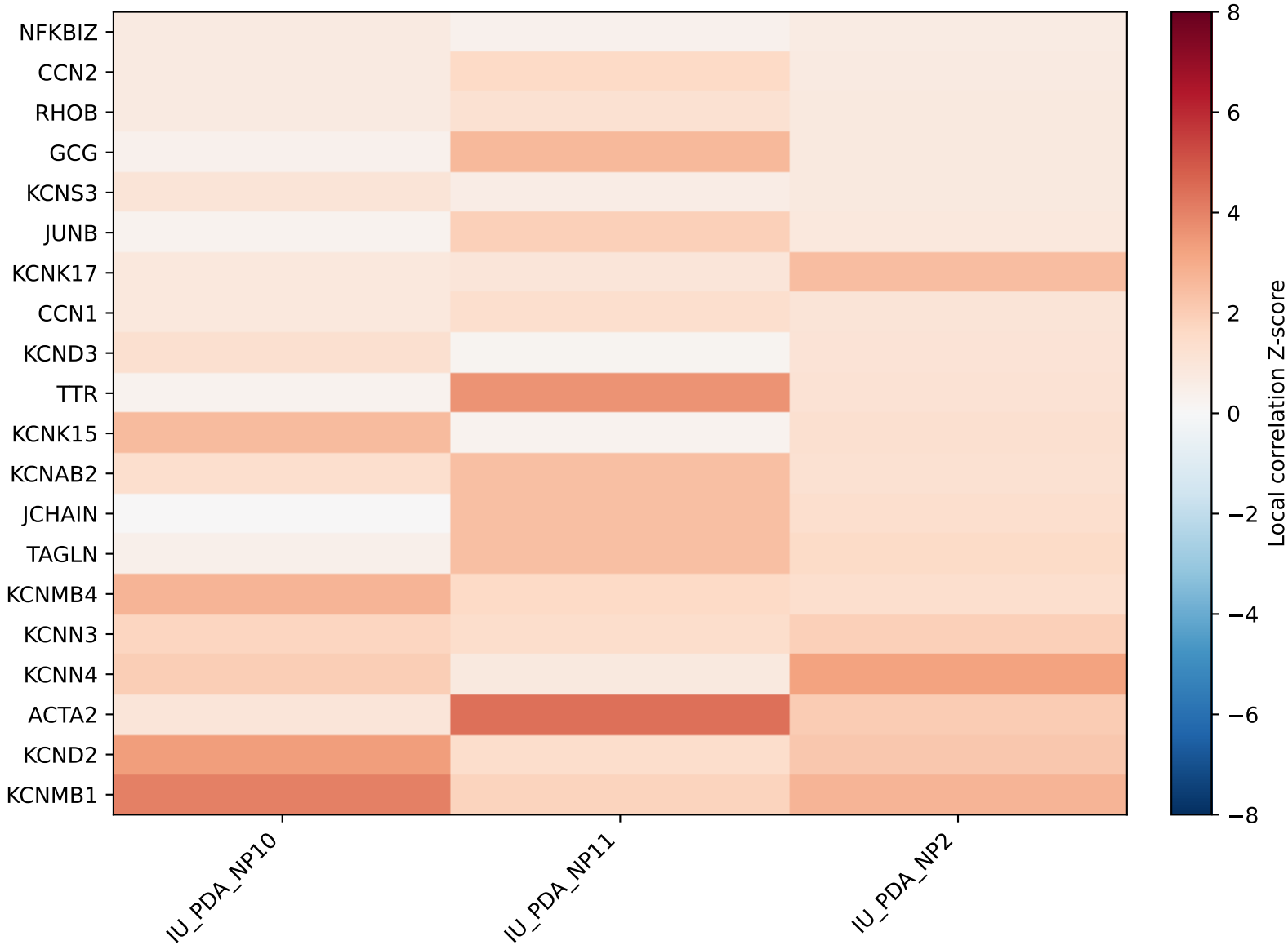
KCNA5 local correlation Z-scores across normal sections
