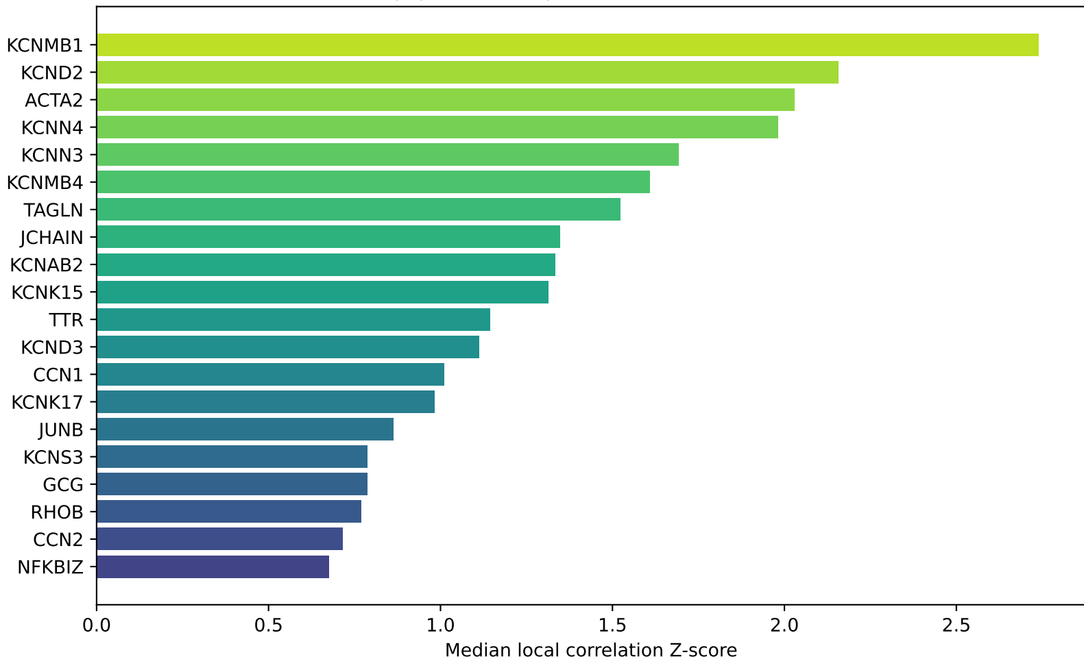
Top genes locally correlated with KCNA5
