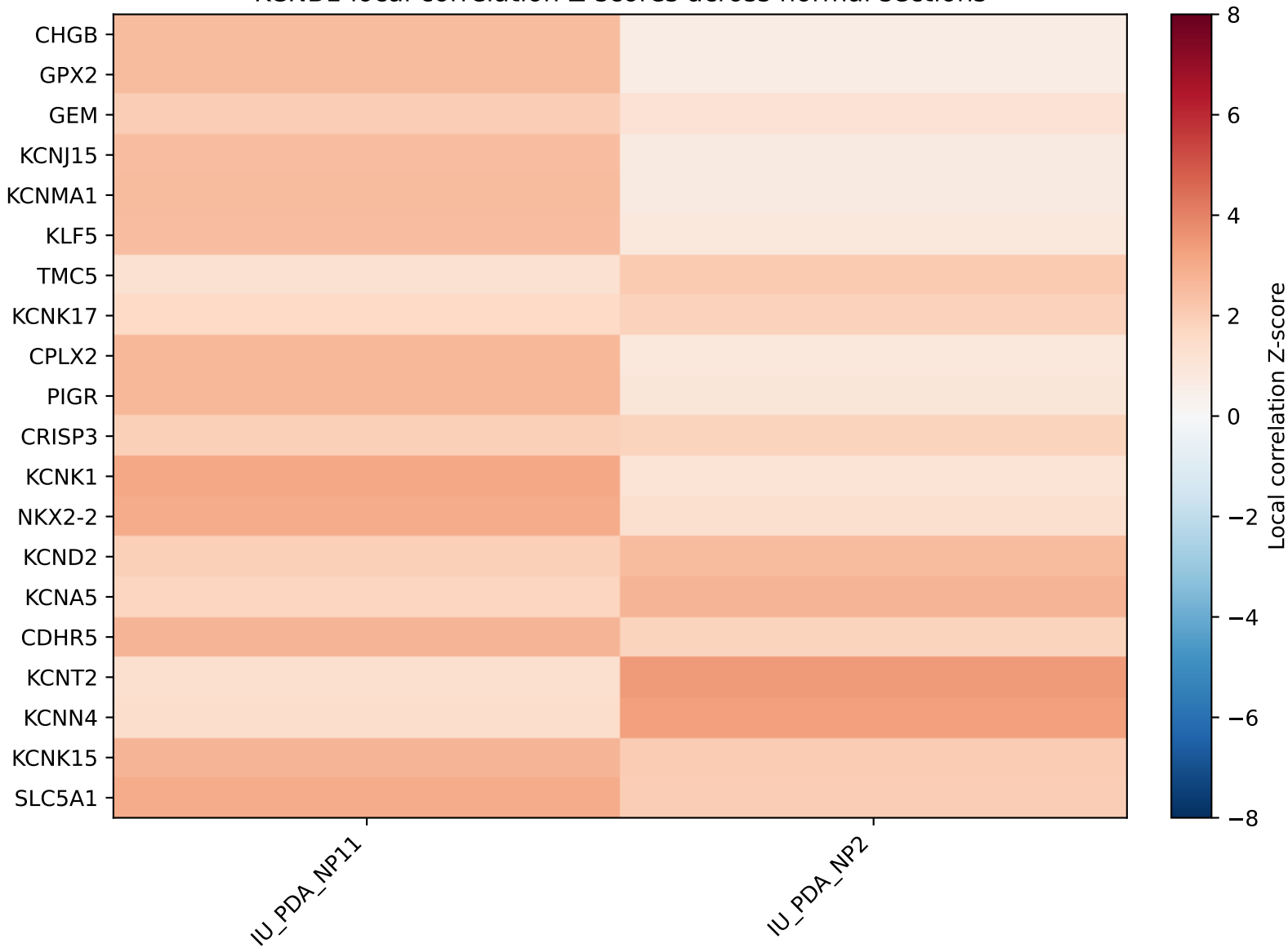
KCNB1 local correlation Z-scores across normal sections
