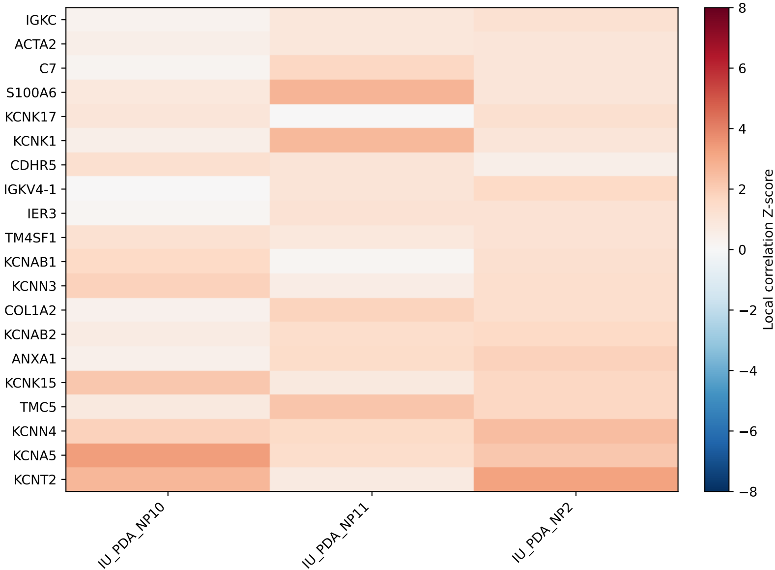
KCND2 local correlation Z-scores across normal sections
