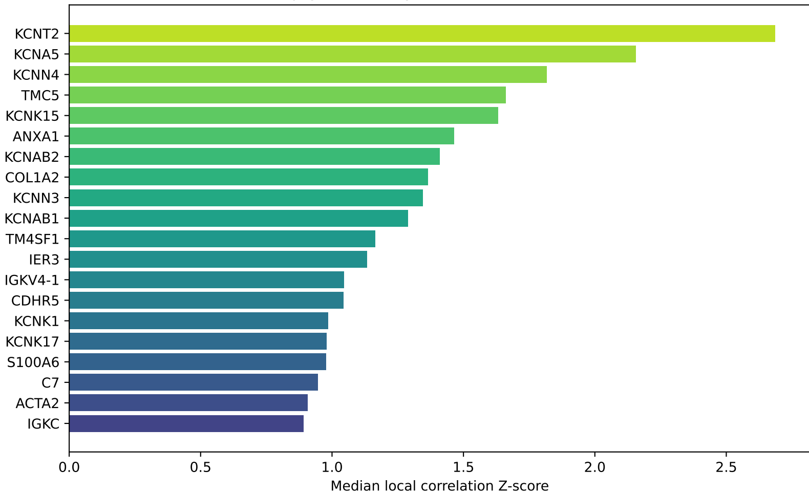
Top genes locally correlated with KCND2
