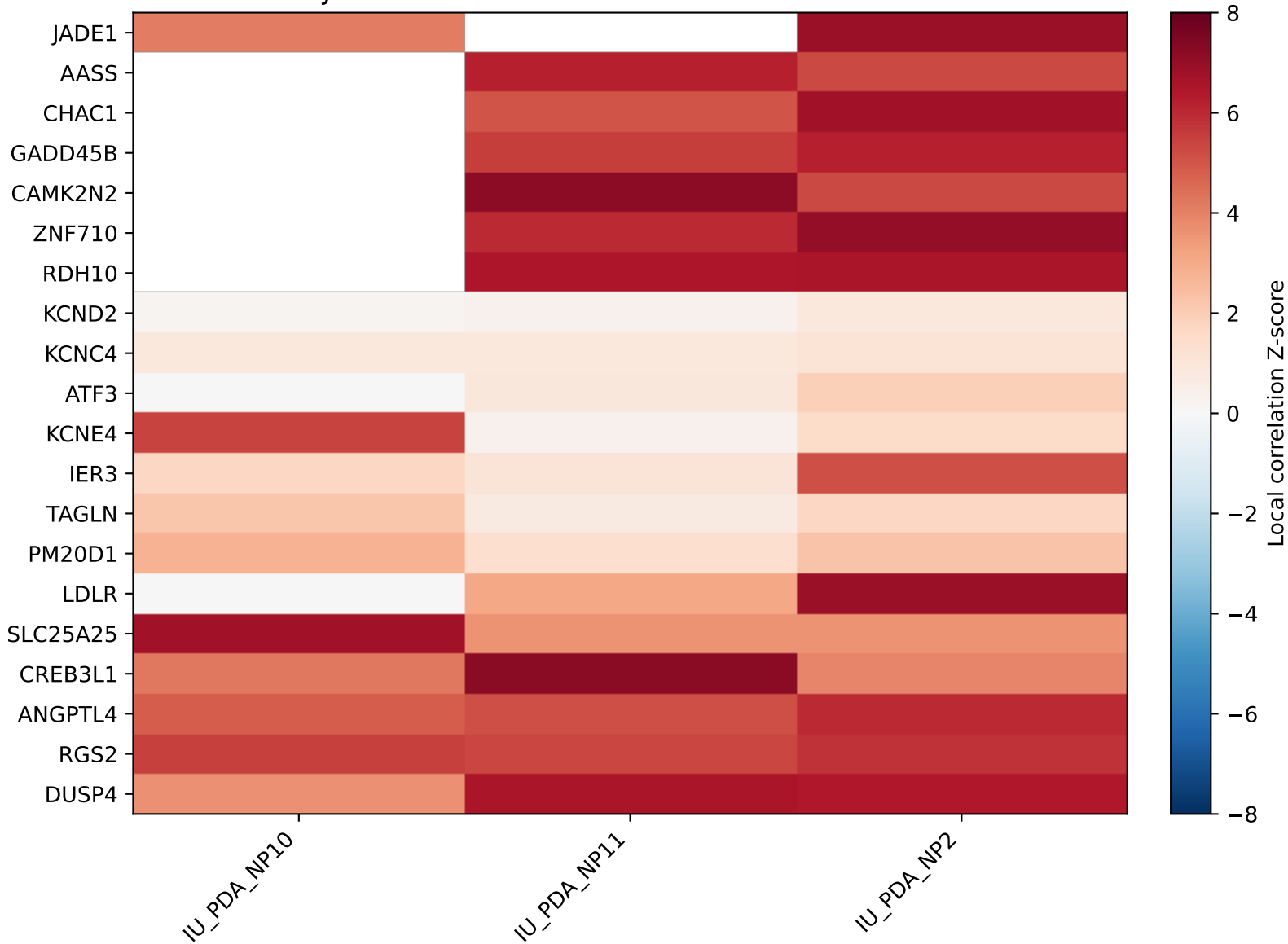
KCNJ8 local correlation Z-scores across normal sections
