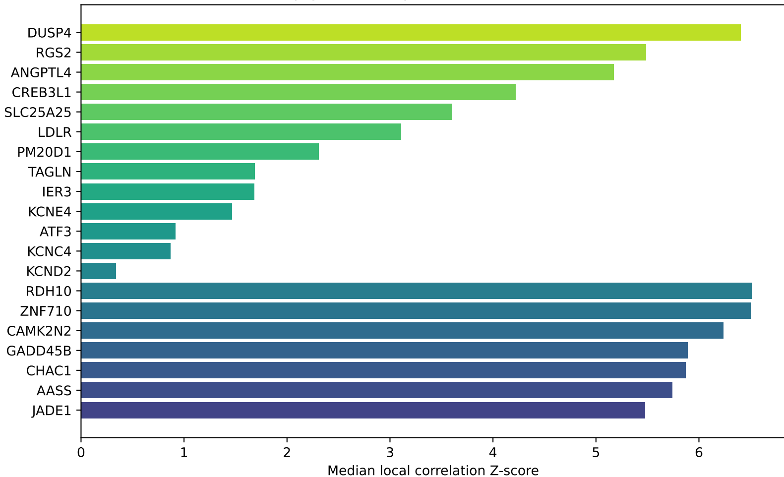
Top genes locally correlated with KCNJ8
