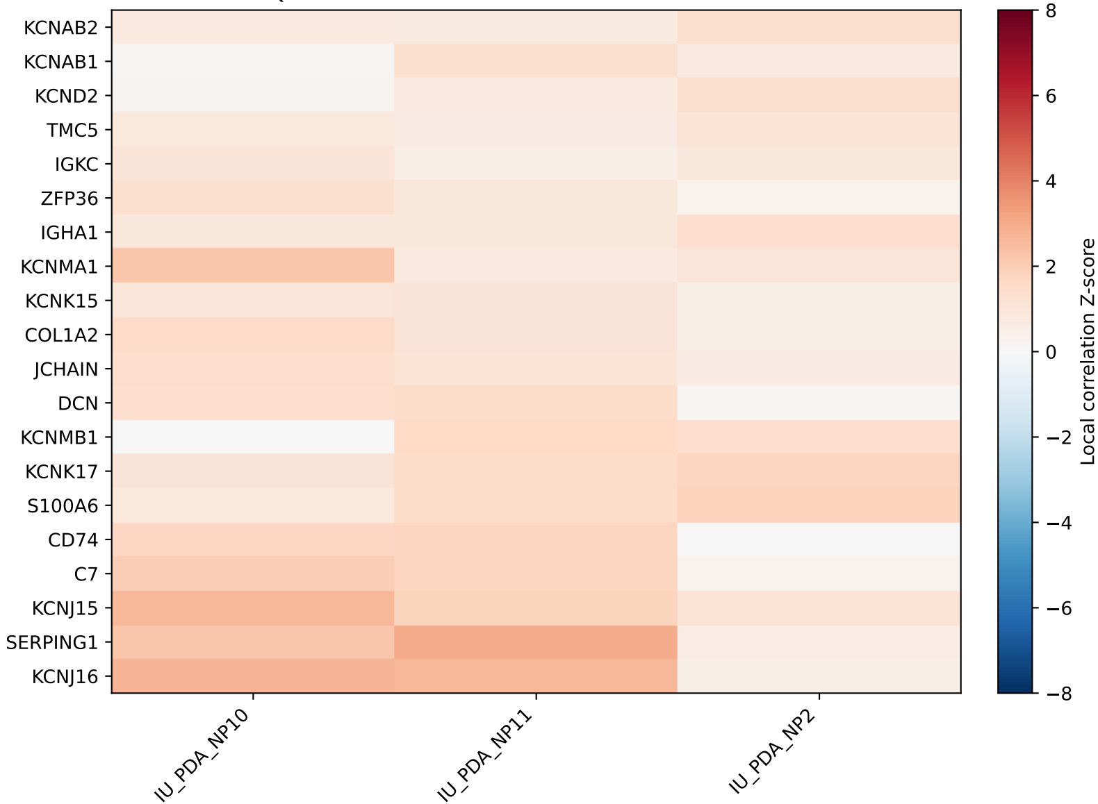
KCNQ4 local correlation Z-scores across normal sections
