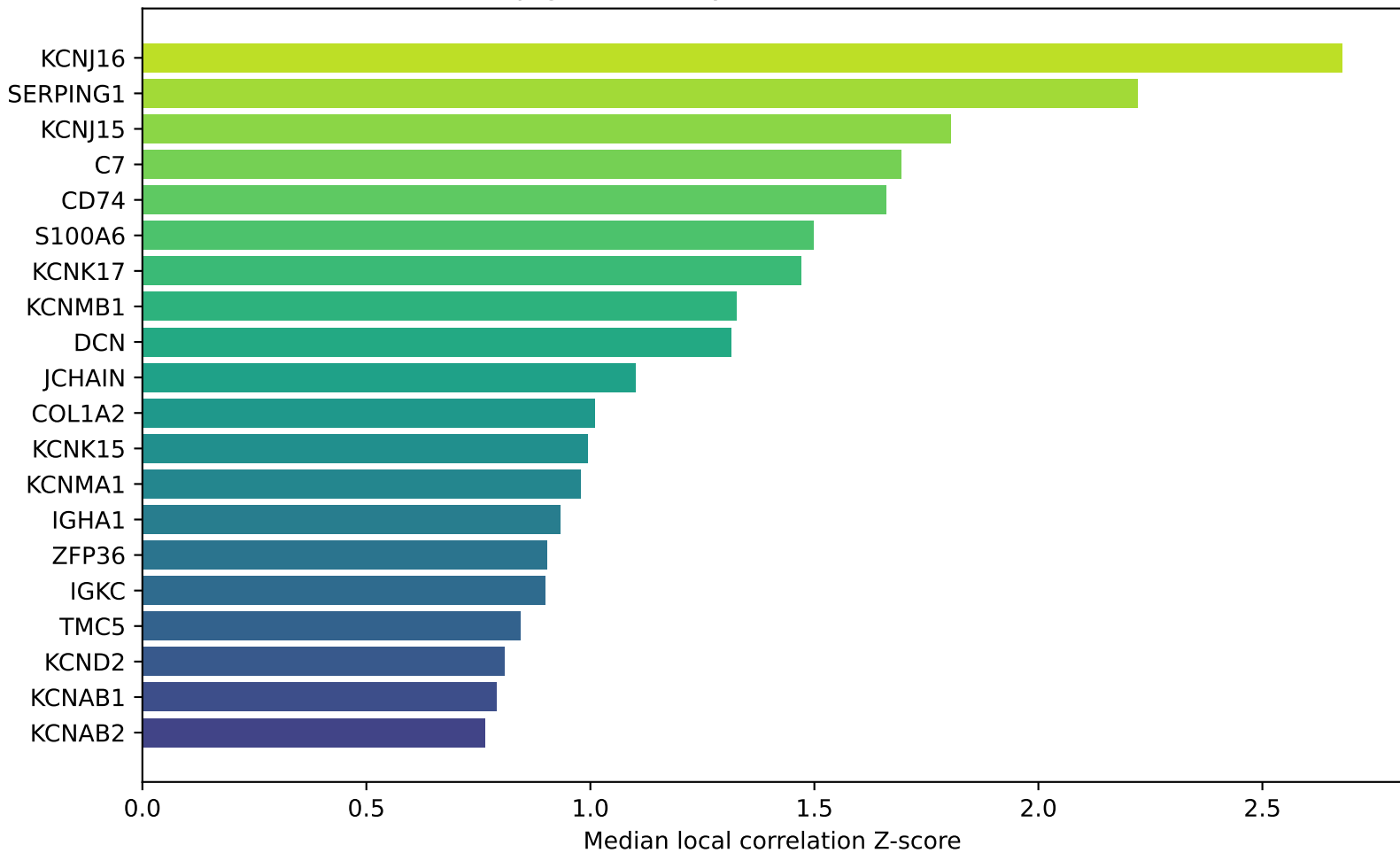
Top genes locally correlated with KCNQ4
