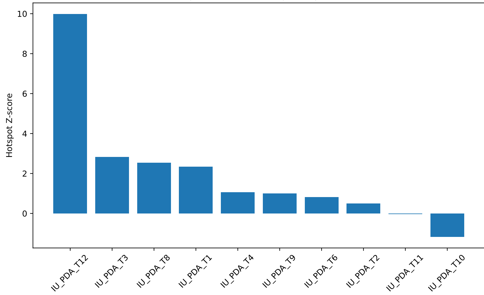
KCNAB2 Hotspot Z-score across primary PDAC sections
