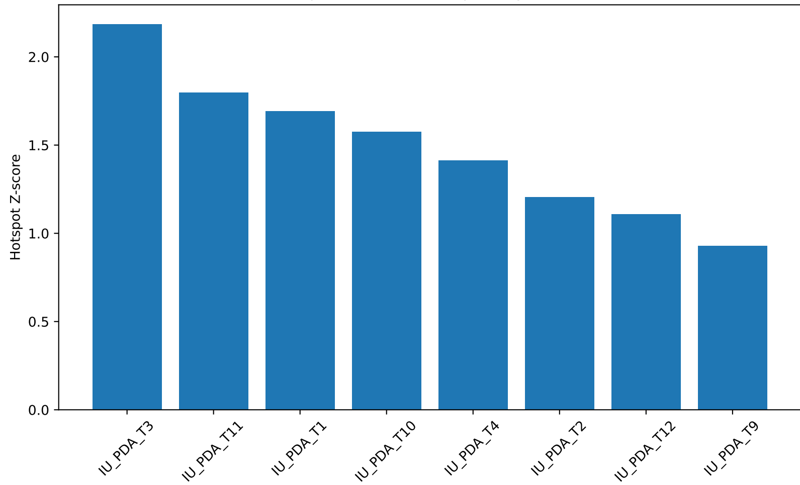
KCNB1 Hotspot Z-score across primary PDAC sections
