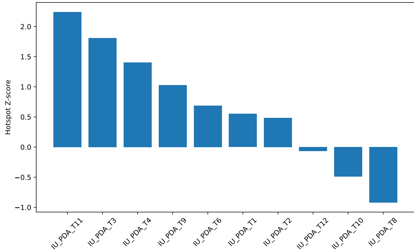
KCNC4 Hotspot Z-score across primary PDAC sections
