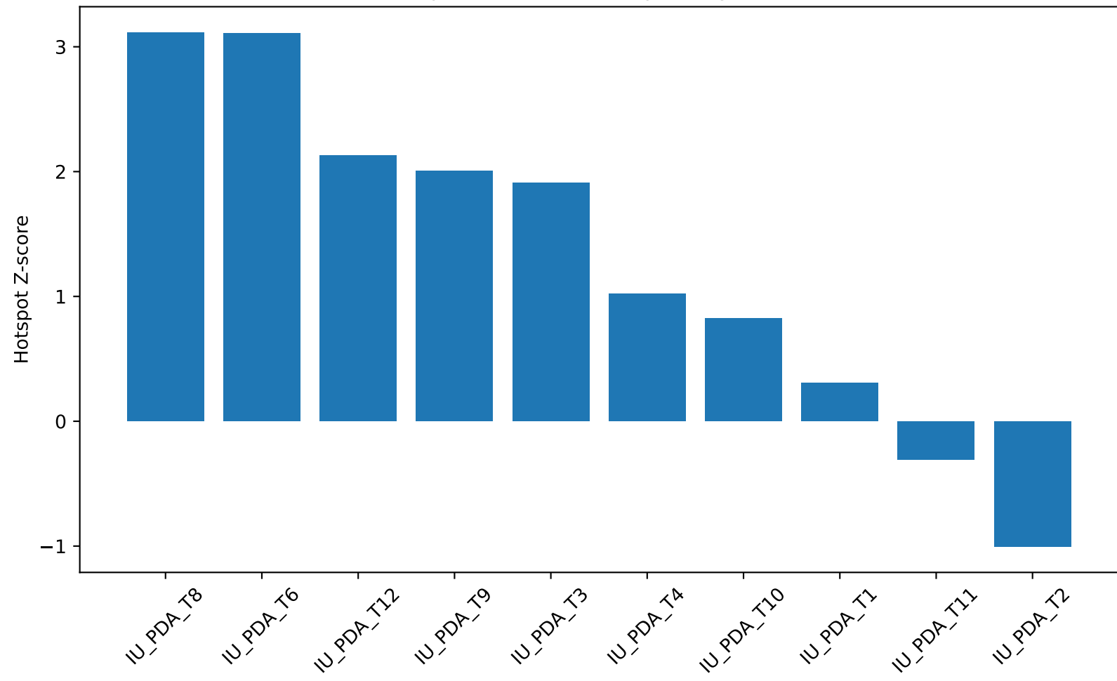
KCNE4 Hotspot Z-score across primary PDAC sections
