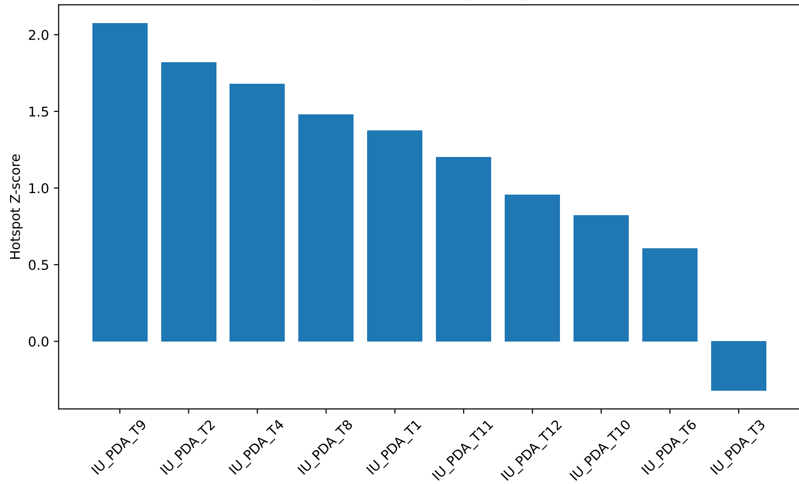
KCNK15 Hotspot Z-score across primary PDAC sections
