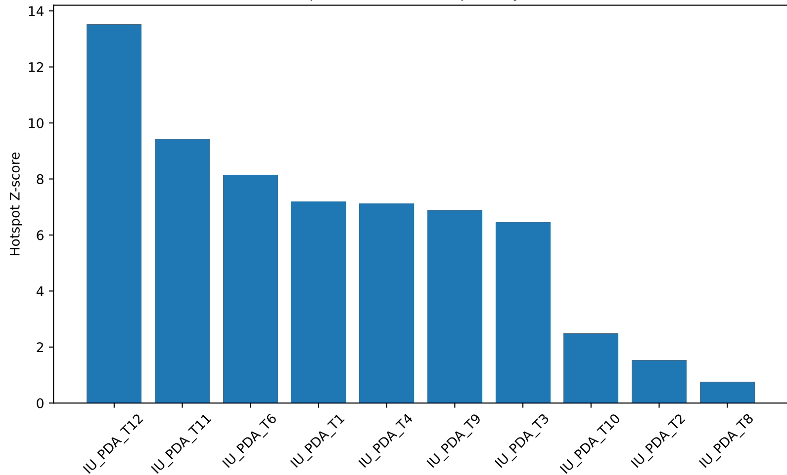
KCNMA1 Hotspot Z-score across primary PDAC sections
