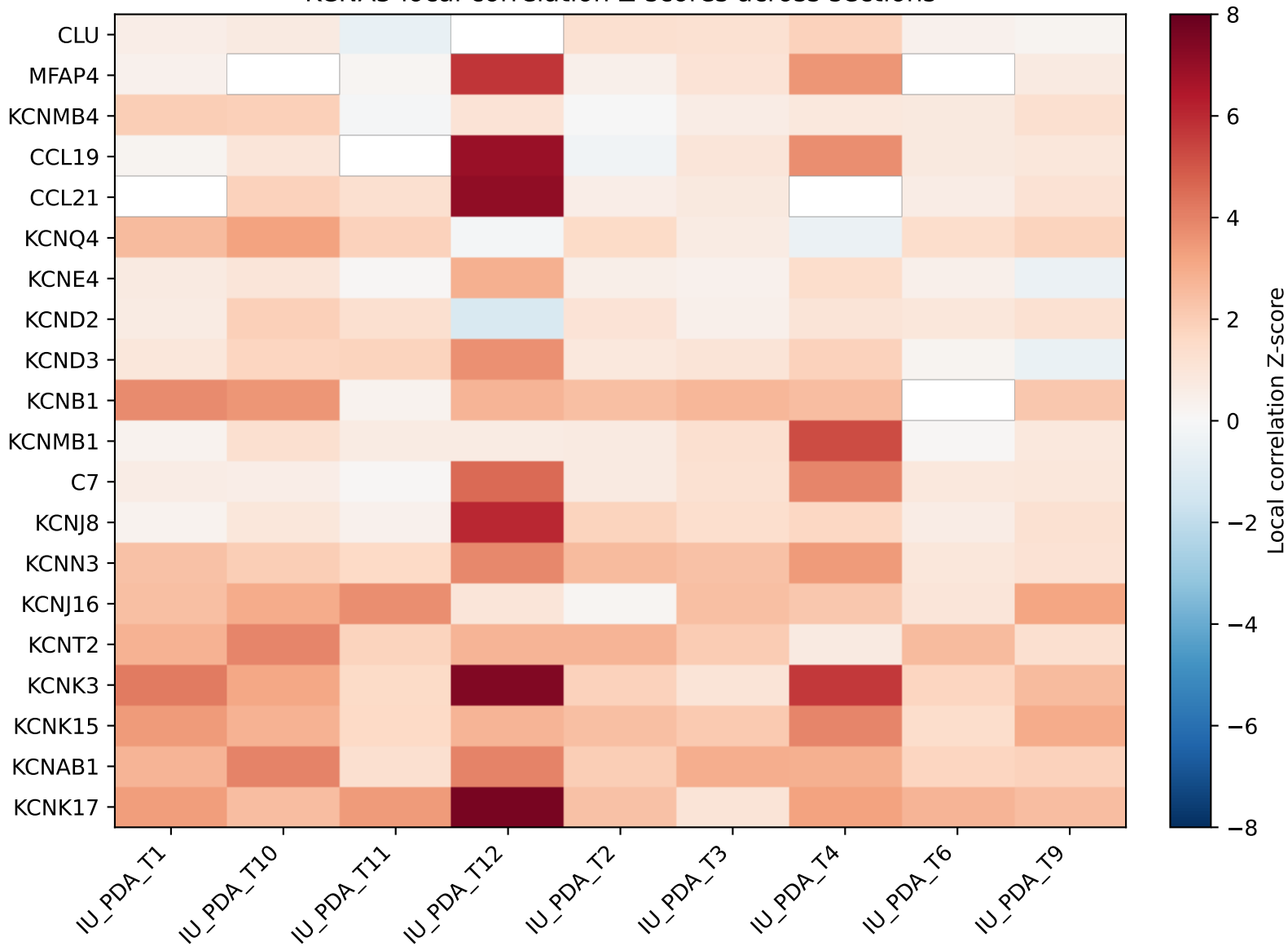
KCNA5 local correlation Z-scores across sections
