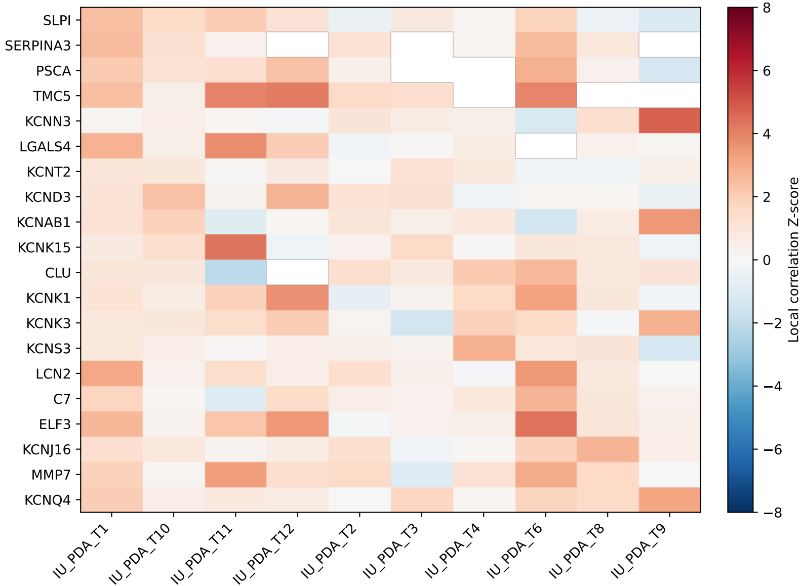
KCNC4 local correlation Z-scores across sections
