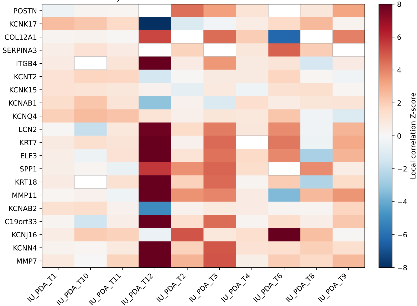
KCNJ15 local correlation Z-scores across sections
