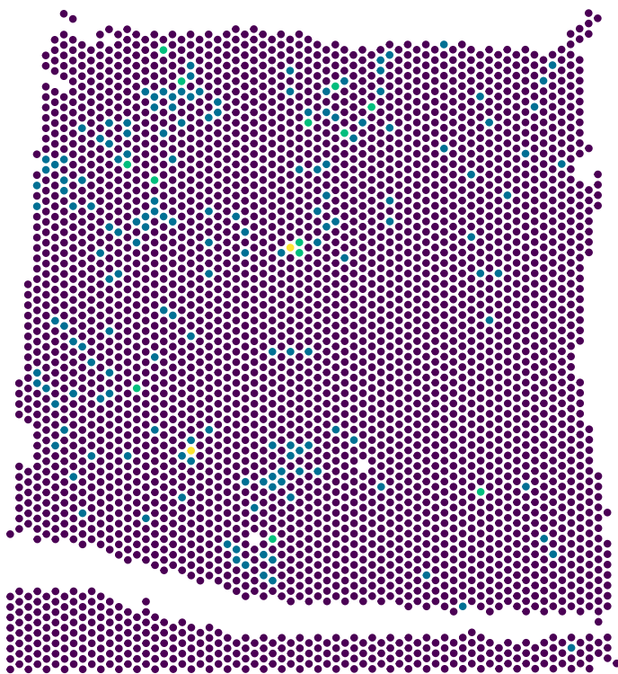
IU_PDA_T4 KCNMA1: C=0.036, Z=7.13, FDR=8.6e-12
