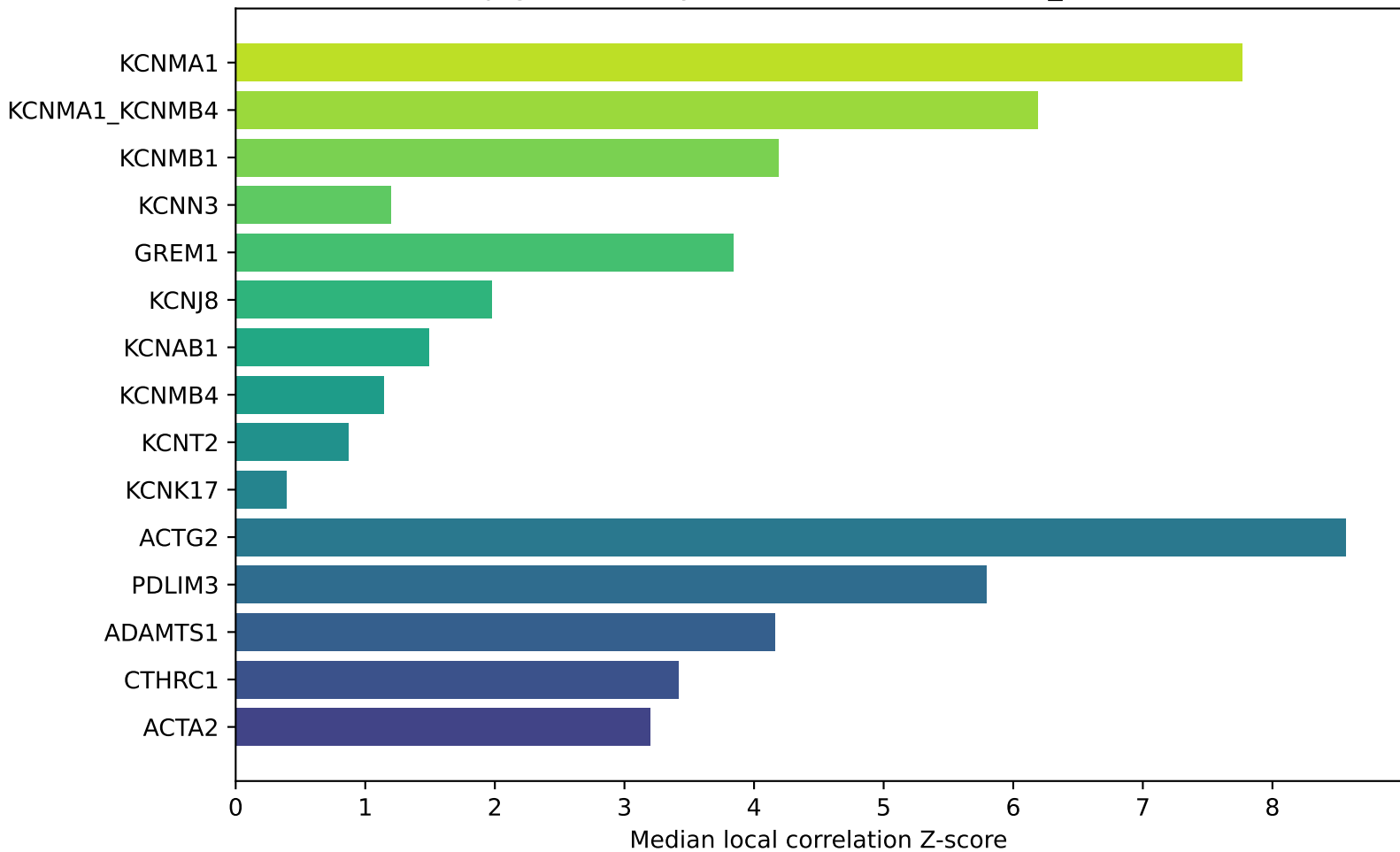
Top genes locally correlated with KCNMA1_KCNMB1
