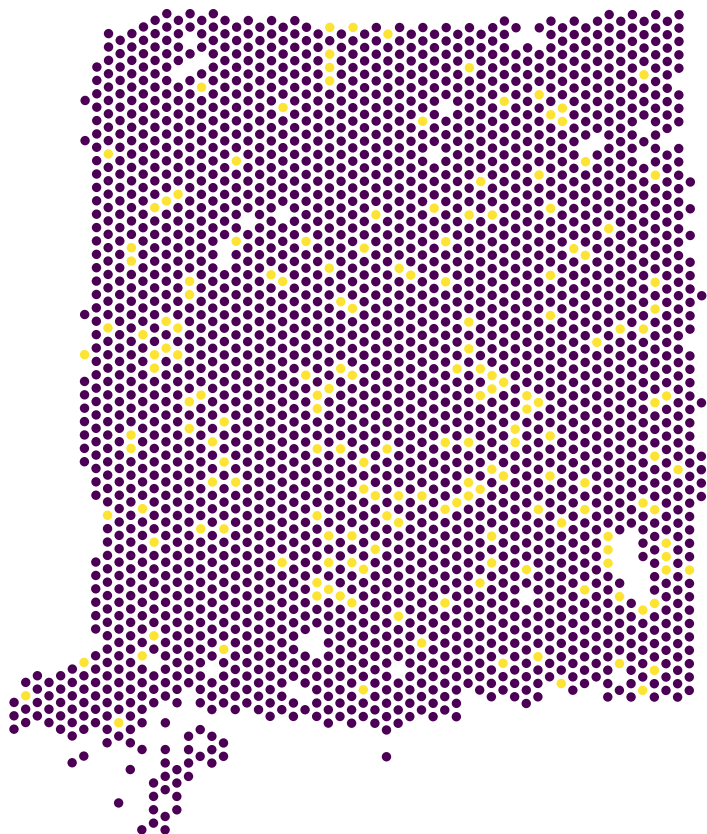
IU_PDA_T10 KCNMA1: C=0.013, Z=2.49, FDR=6.5e-02
