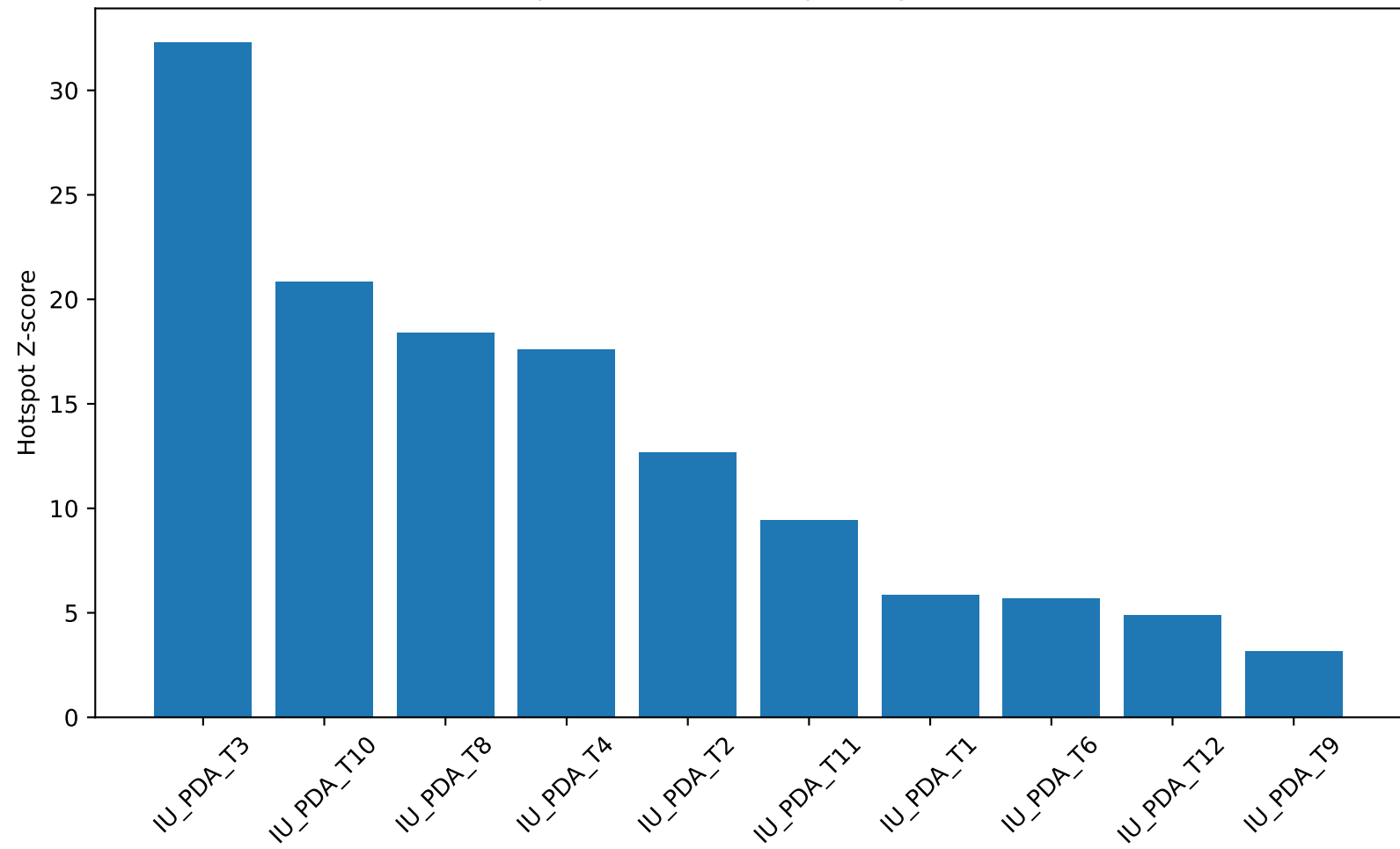
ACTA2 Hotspot Z-score across primary PDAC sections
