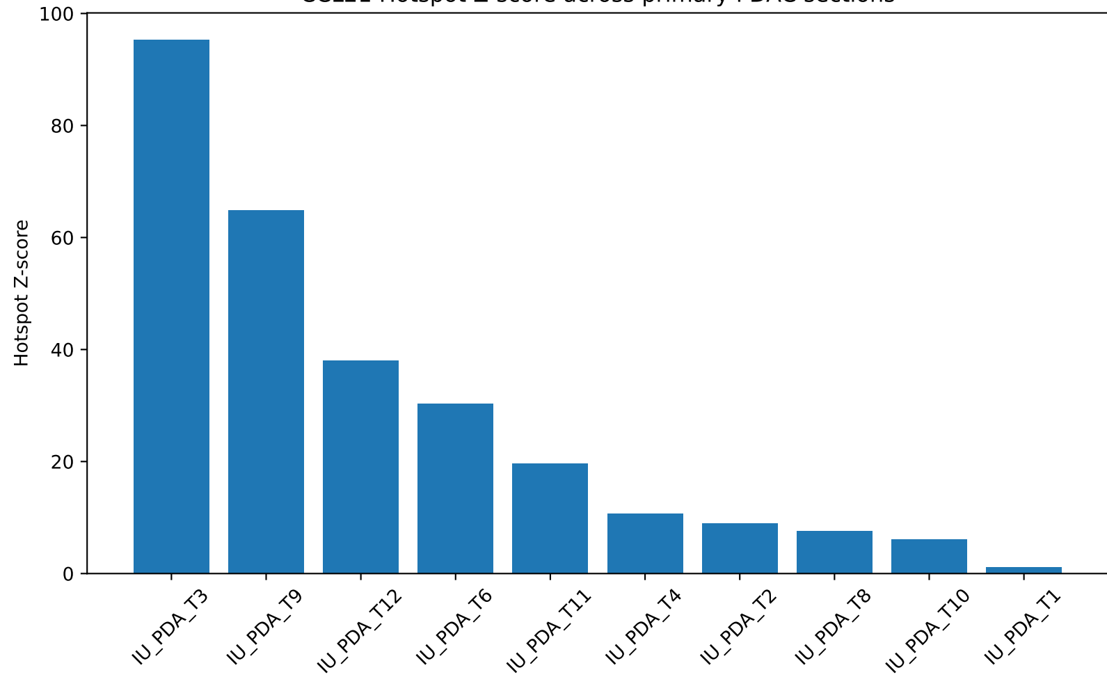
CCL21 Hotspot Z-score across primary PDAC sections
