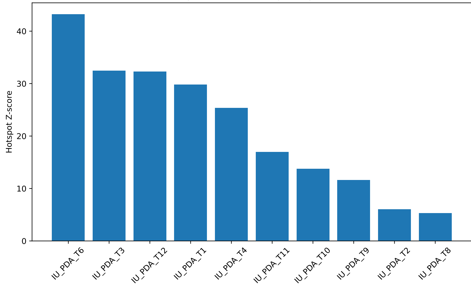
COL12A1 Hotspot Z-score across primary PDAC sections
