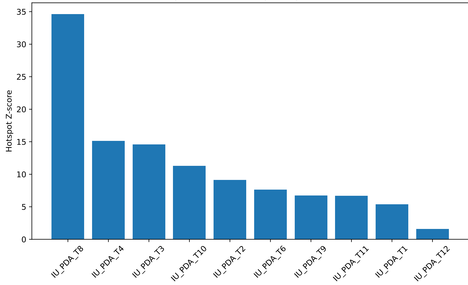
DCN Hotspot Z-score across primary PDAC sections
